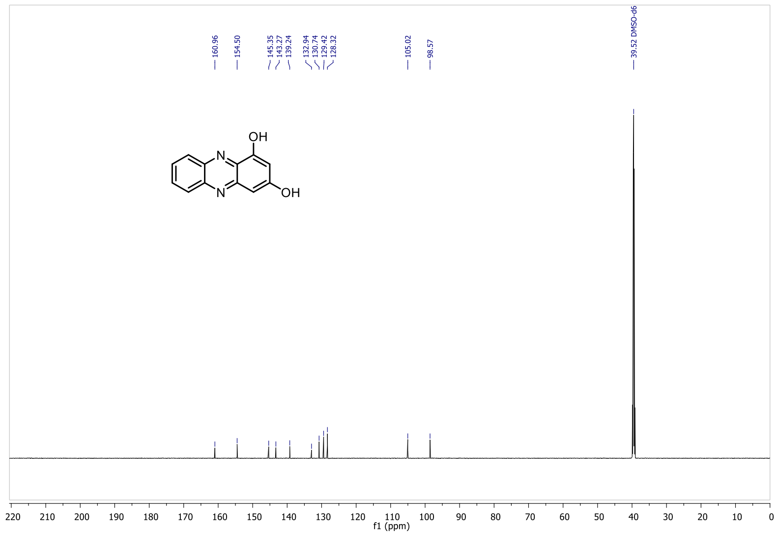
^{13}\text{C} NMR of 1,3-dihydroxyphenazine in \text{d}_6 -DMSO.
